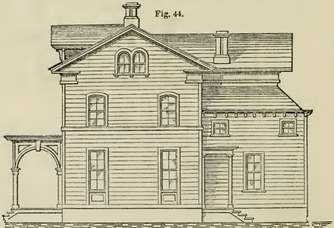
SIDE ELEVATION.
